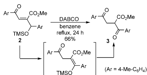
Scheme 3. Conversion of product 2 into product 3 .
