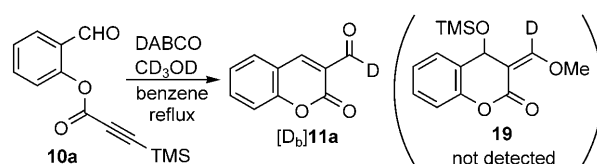
Scheme 11. Coumarin-forming reaction in the presence of [D] 4 MeOH .
