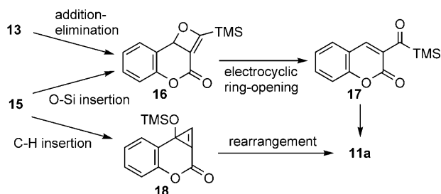
Scheme 9. Alternative reaction pathways for formylcoumarin formation.
