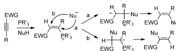
Scheme 1. Phosphine-catalyzed \alpha - or \beta -activation of alkynes towards nucleophiles.
