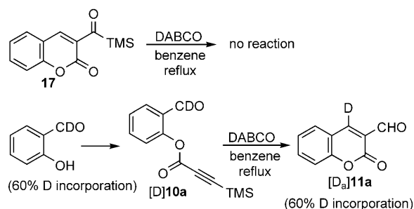
Scheme 10. Experiments conducted to clarify the reaction mechanism of formylcoumarin formation.
