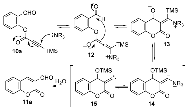
Scheme 8. A plausible reaction mechanism for the formation of the formylcoumarins.
