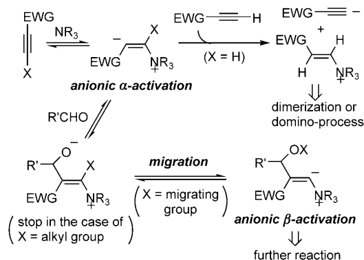
Scheme 2. Our new concept for the consecutive \alpha - and \beta -activation of alkynes towards electrophiles.
