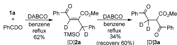
Scheme 7. Experiments using benz[D]aldehyde.
